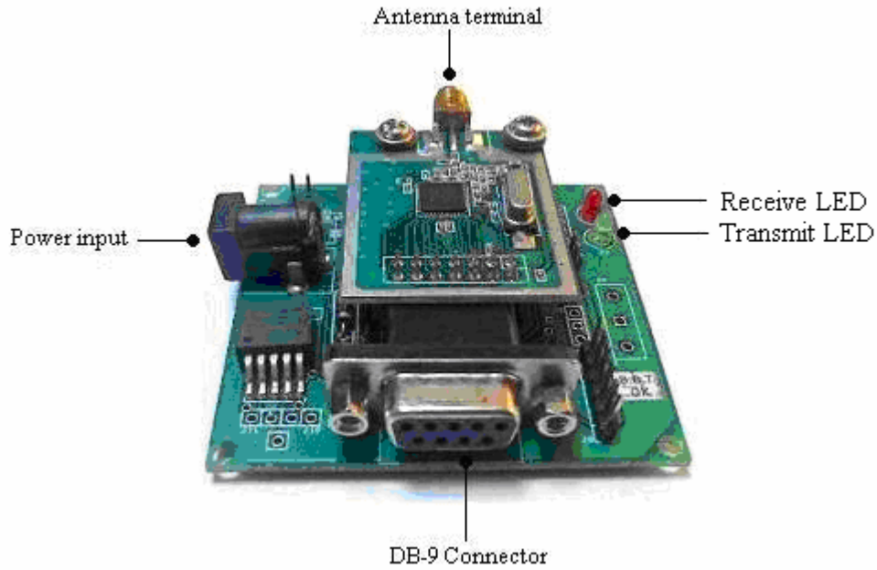
Figure 2: RDSRF-232-T3FZ connection diagram
