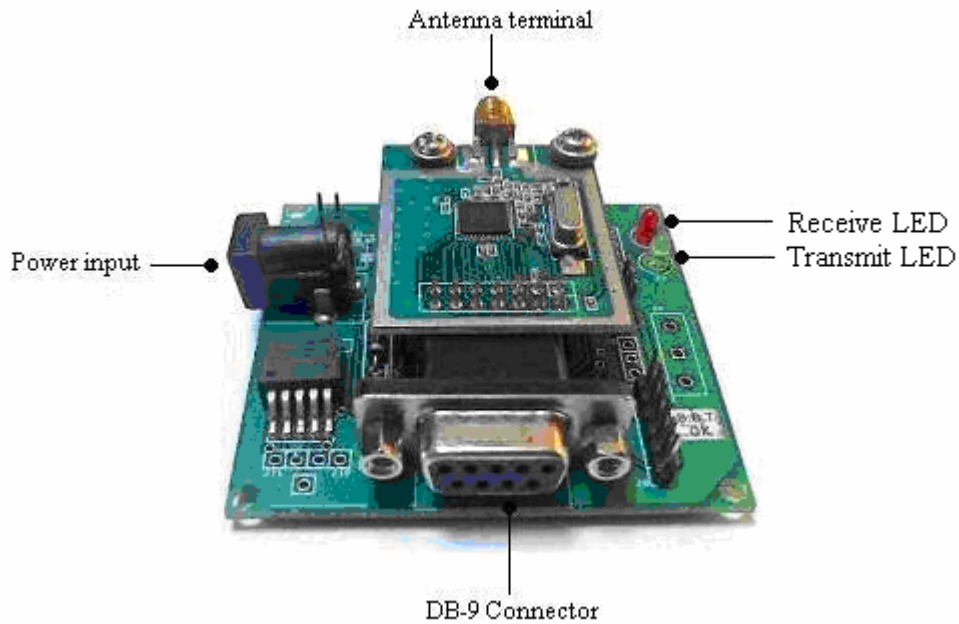
Figure 2: RDSRF-232-T8FZ connection diagram
