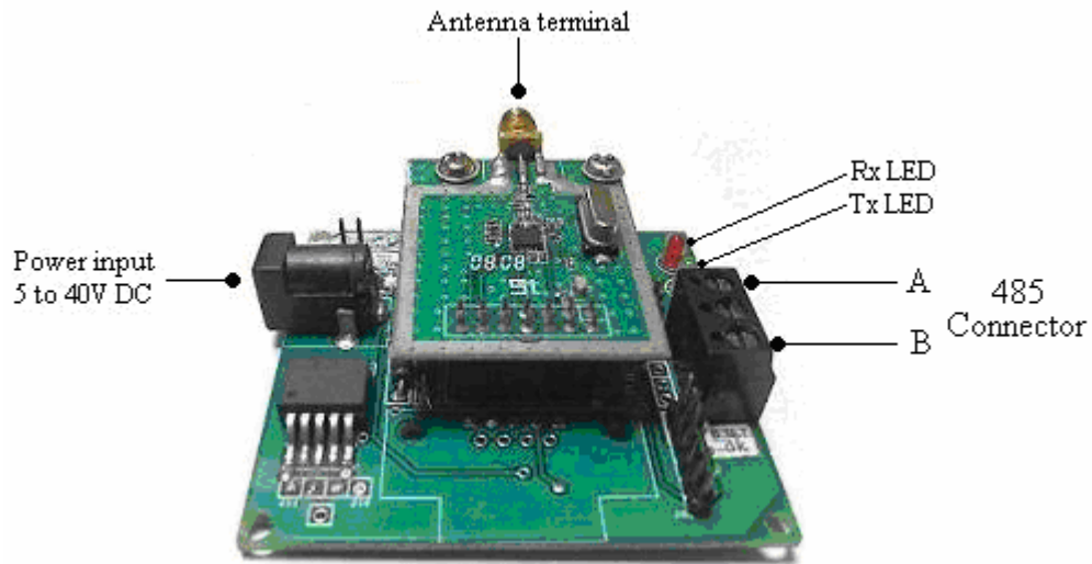
Figure 2: RDSRF-485-T24FZ connection diagram
