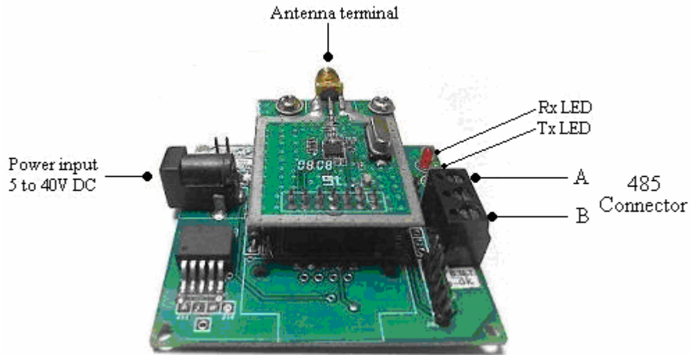
Figure 2: RDSRF-485-T4FZ connection diagram
